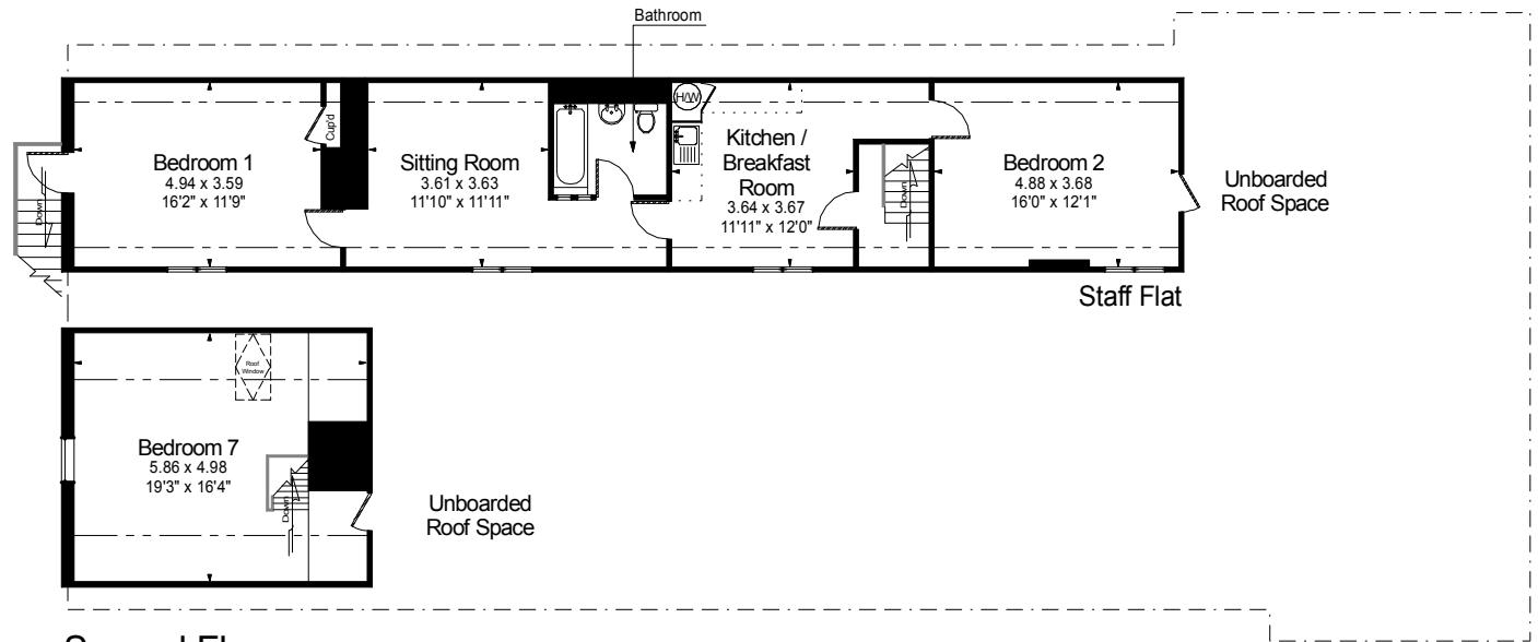
Second Floor
